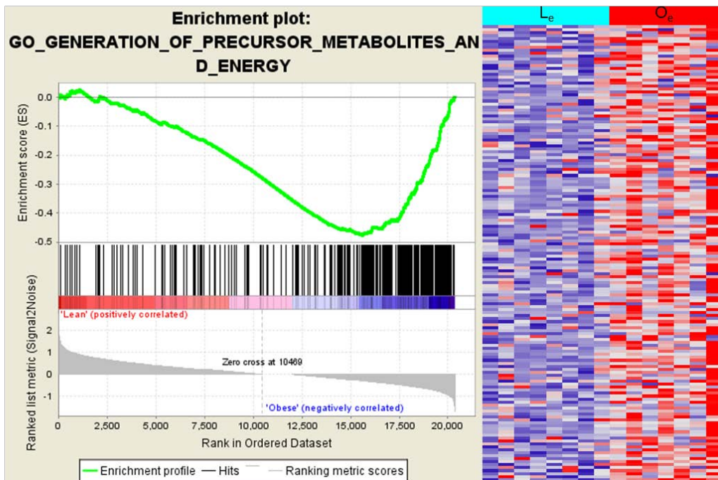
Figure S2. GSEA analysis of LO-DEGs.
